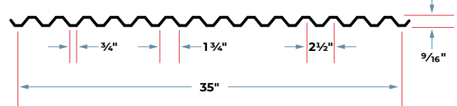
9/16" FORM DECK
