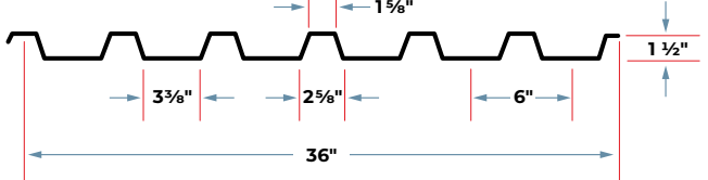
1.5" FORM DECK
