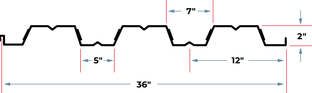
2" COMPOSITE DECK
