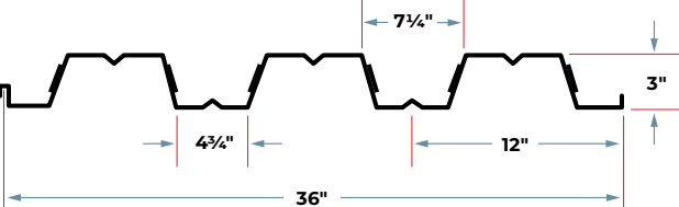
3" COMPOSITE DECK
