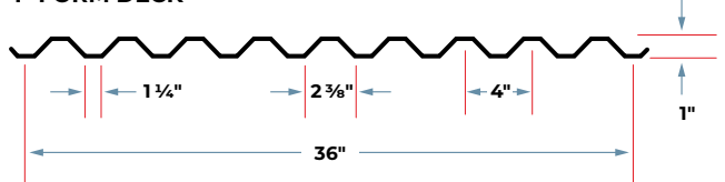
1" FORM DECK
