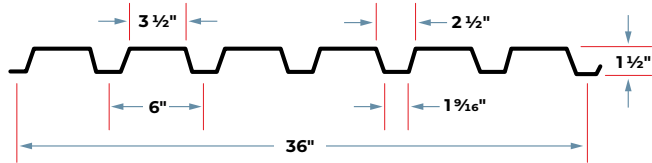
B-DECK
