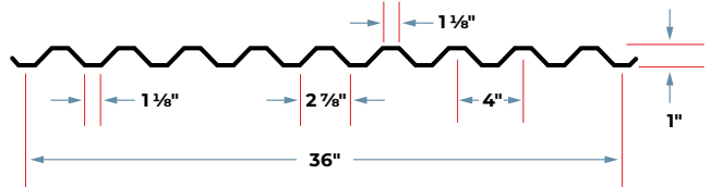
1" ROOF DECK
