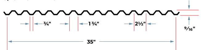
9/16" FORM DECK
