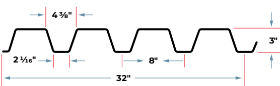
N-DECK
