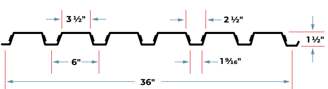
1.5" COMPOSITE DECK
